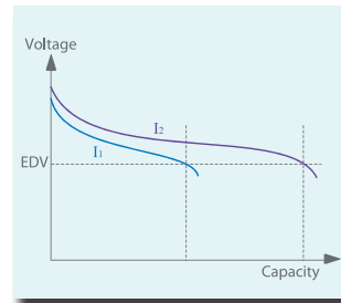
Capacity Testing
