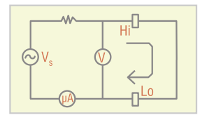
If circuit shorted : C_m \gg C_x
