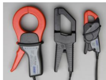
DENT's popular 1000A, 500A and 150A Clamp-On style Current Transformers. All DENT CTs are interchangeable on the ELITE pro ™, allowing a level of flexibility not found on other commercial power meters.
