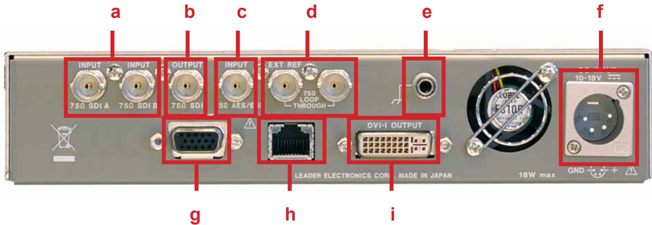
LV7330 Rear Panel
